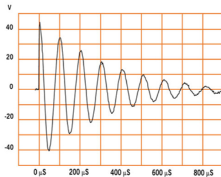
FIG. 1 – DAMPED SINUSOIDAL PULSE, (10 kHz) INTO AN OPEN CIRCUIT
