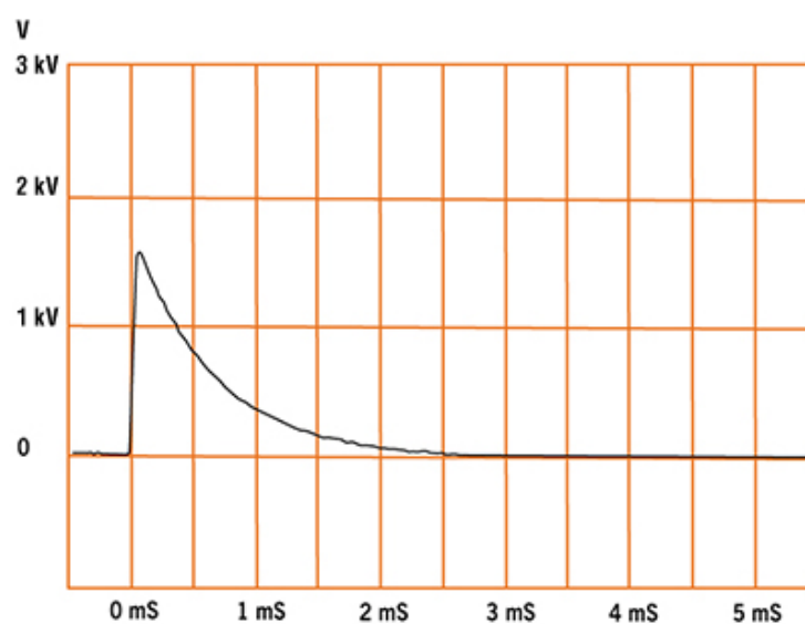
FIG. 2 – DOUBLE EXPONENTIAL PULSE INTO AN OPEN CIRCUIT
