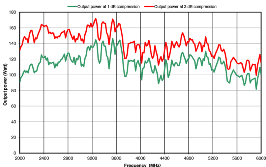
UX100 POWER AMPLIFIER 100W / 2 GHz - 6 GHz
