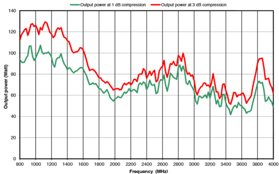
SW65 POWER AMPLIFIER 65W / 800 MHz - 4 GHz
