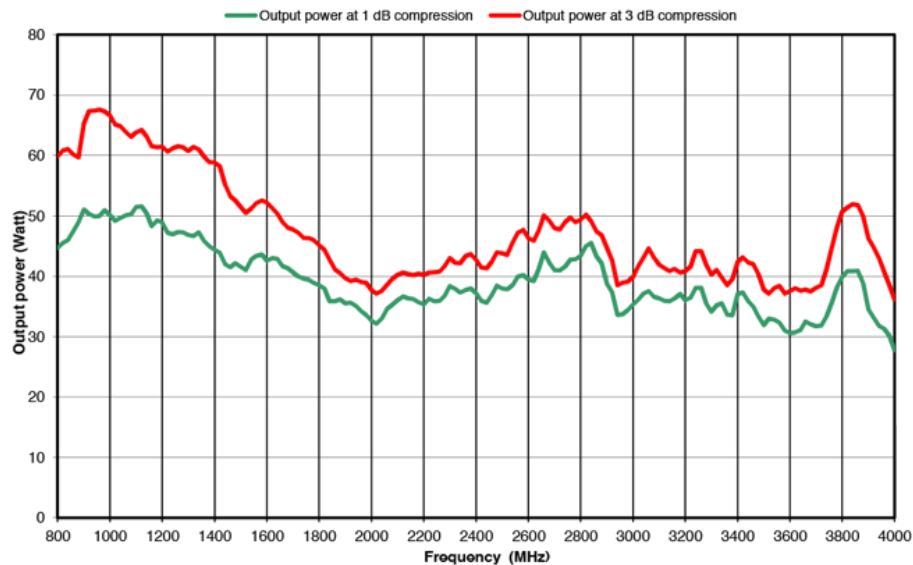
SW35 POWER AMPLIFIER 35W / 800 MHz - 4 GHz
