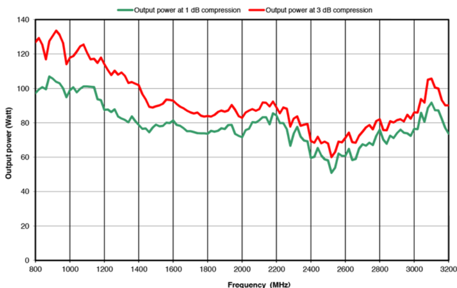
SV70 POWER AMPLIFIER 70W / 800 MHz - 3200 MHz
