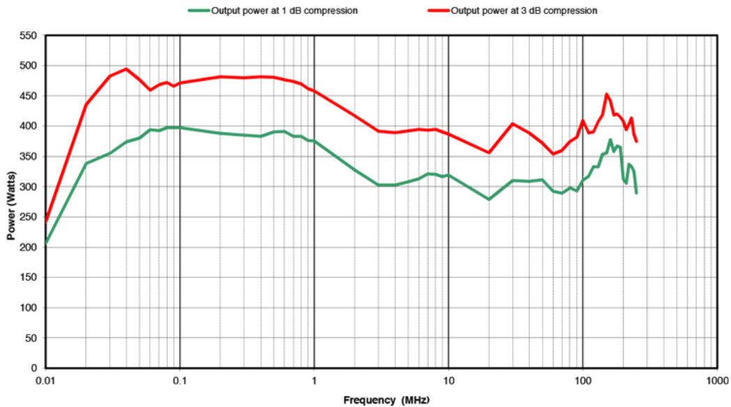
DP300 POWER AMPLIFIER 300W / 10 KHz - 250MHz
