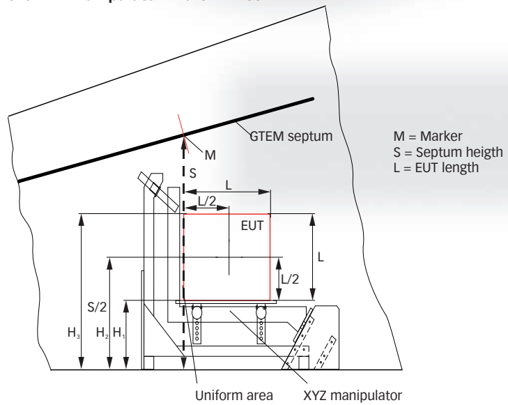
Position of the XYZ manipulator in a GTEM cell
