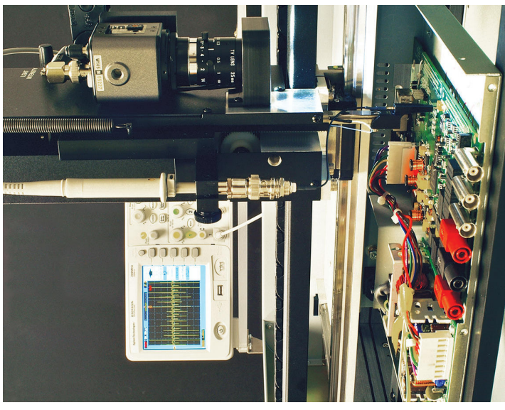
Oscilloscope probe mounted to a custom holder on a Huntron Access Prober allowing for higher frequency measurements.
