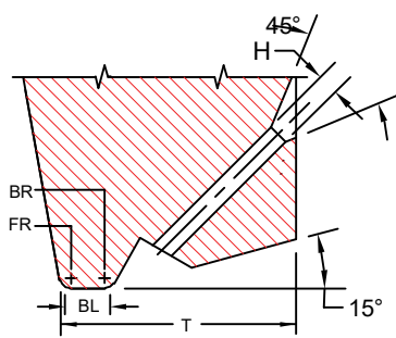
45° Hole Angle
